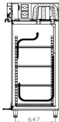
SECTION I-I
