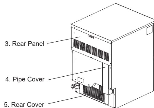
Rear view before removal
